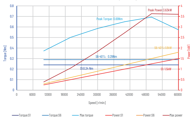
Motor Power and Torque Diagram
