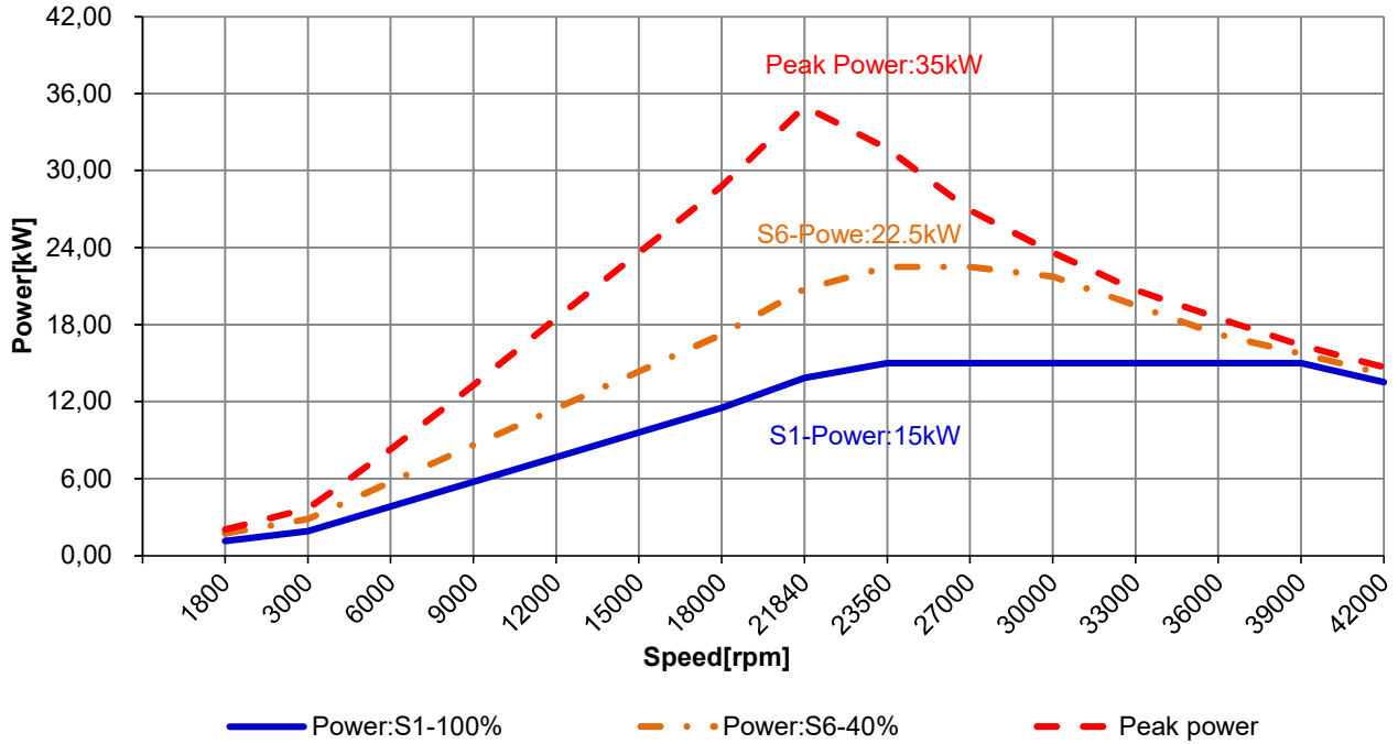
Power Diagram (Cycle time:2 min)
