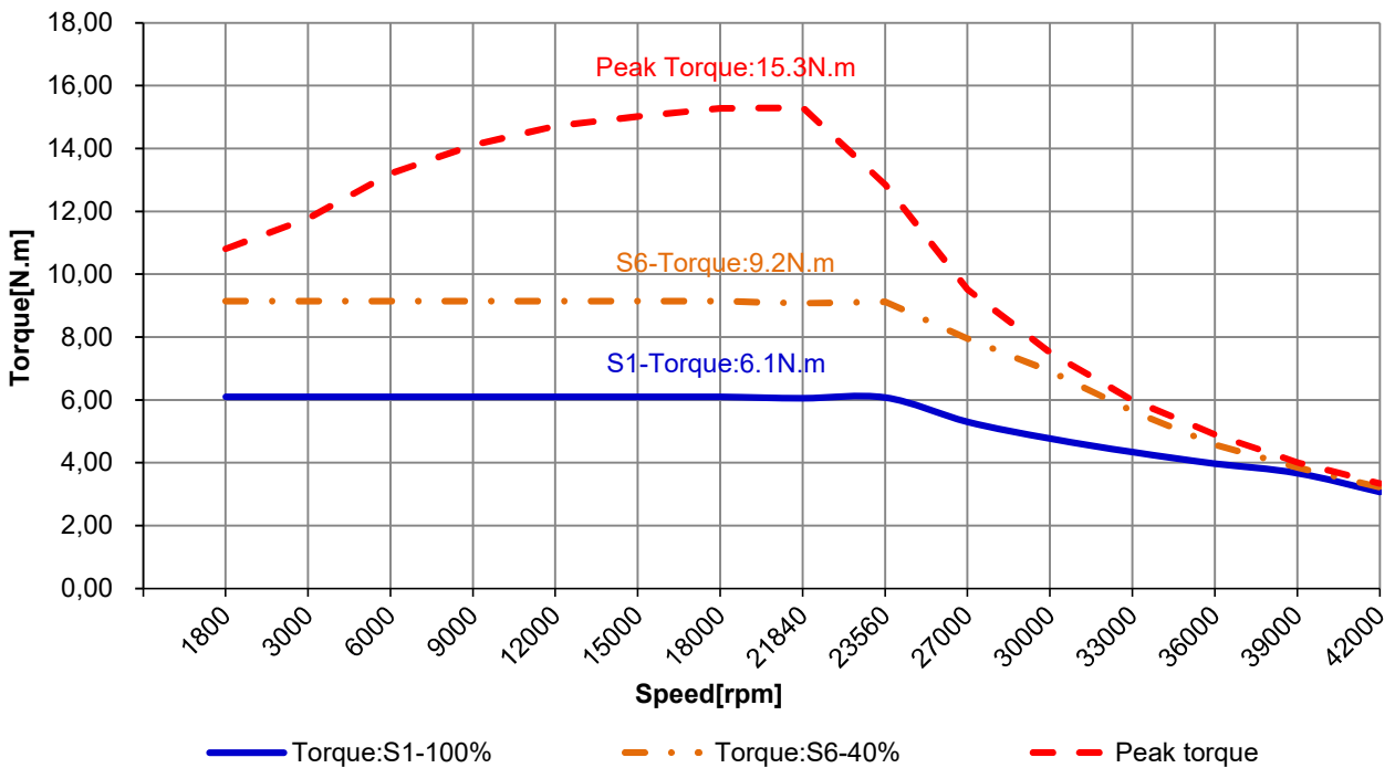
Torque Diagram (Cycle time:2 min)
